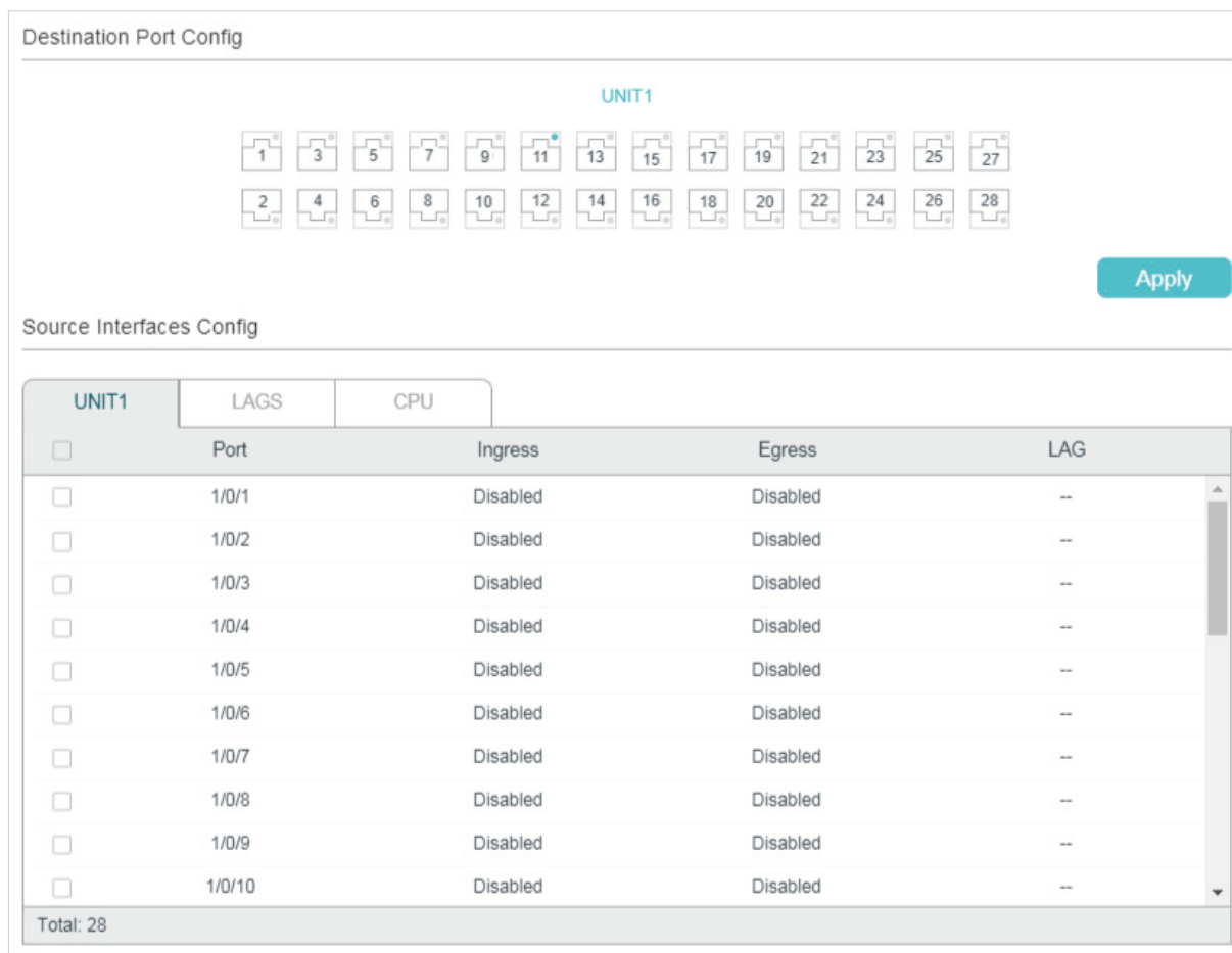
Figure 1-2 Configure the Mirroring Session
