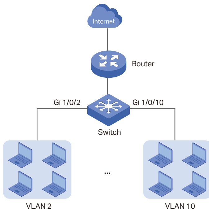
Figure 3-1 Network Topology
