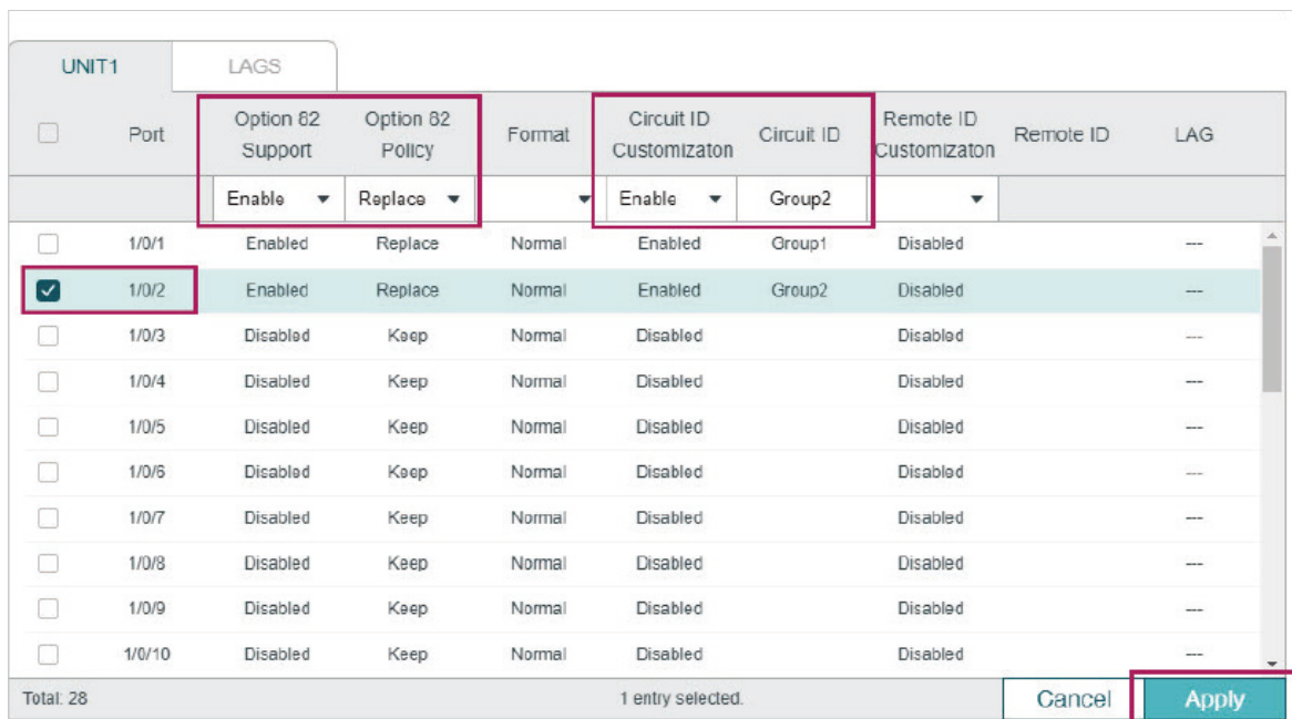
Figure 5-35 Configuring Port 1/0/2
