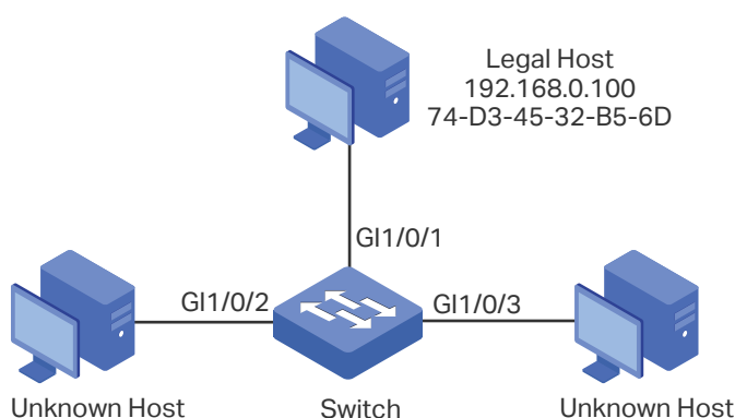
Figure 5-6 Network Topology
