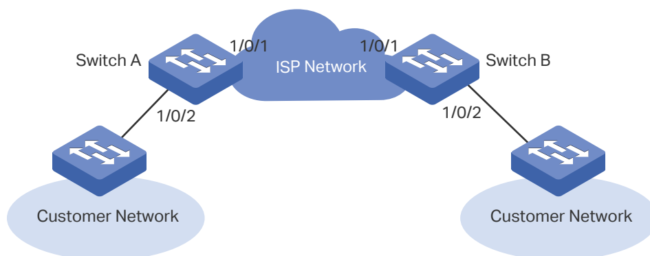
Figure 3-1 Network Topology
