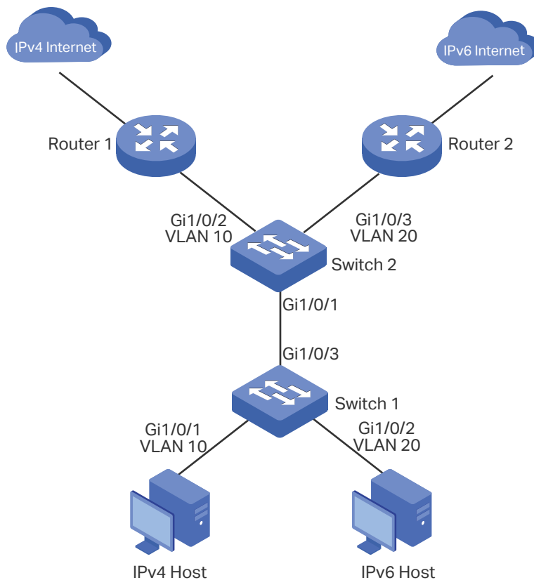
Figure 3-1 Network Topology
